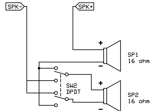
OPTIONAL SPEAKER PHASE REVERSAL
