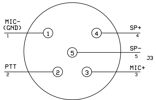
Switchcraft TA5 (Female Pins) Rear View
