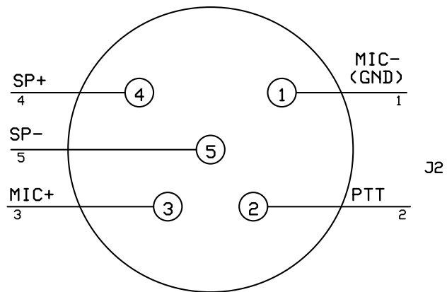
Switchcraft TB5 (Male Pins) Rear View
